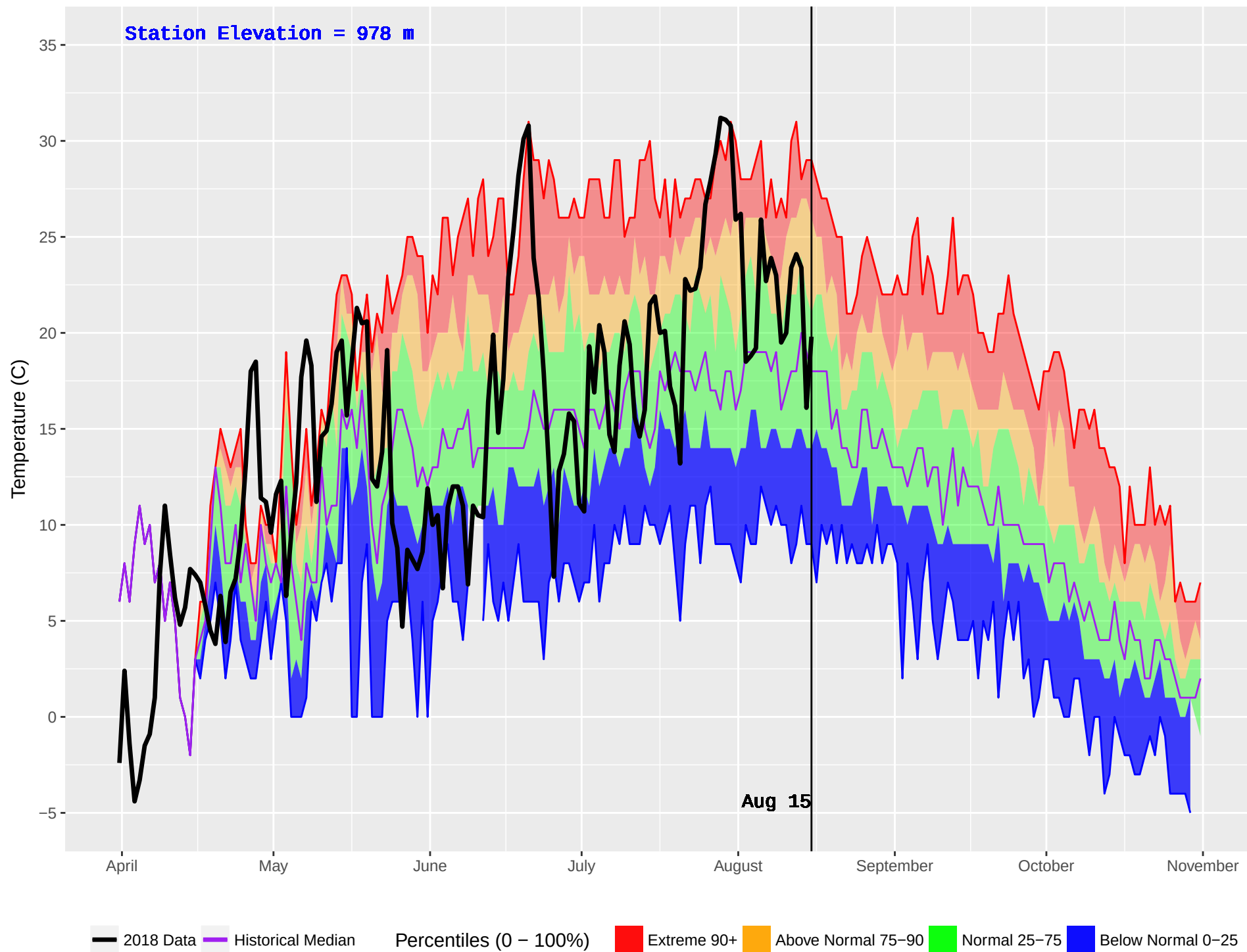
NILKITKWA (172) : Historical (1986–2016) and Current (2018) Daily Temperature
