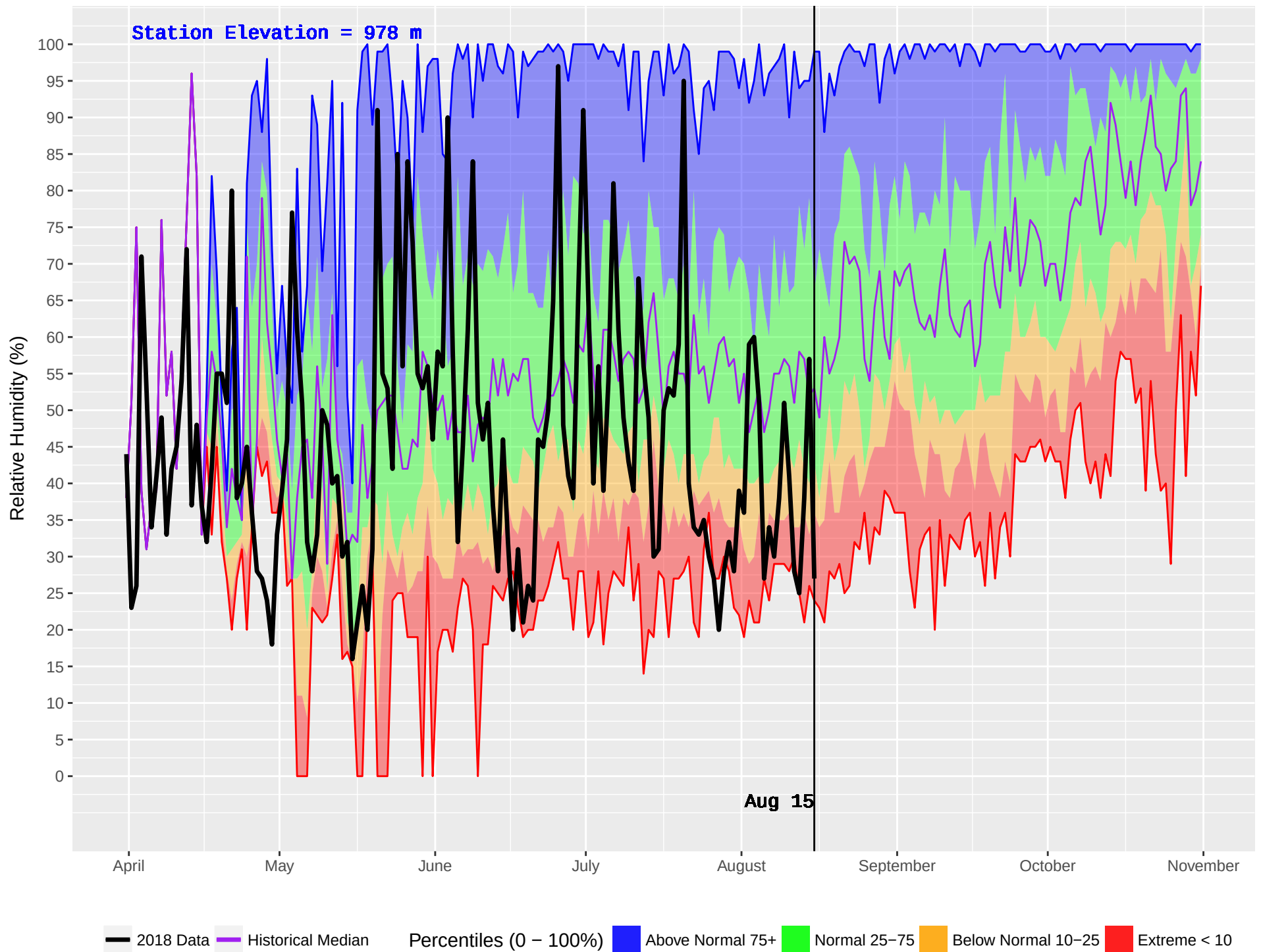
NILKITKWA (172) : Historical (1986–2016) and Current (2018) Daily Relative Humidity
