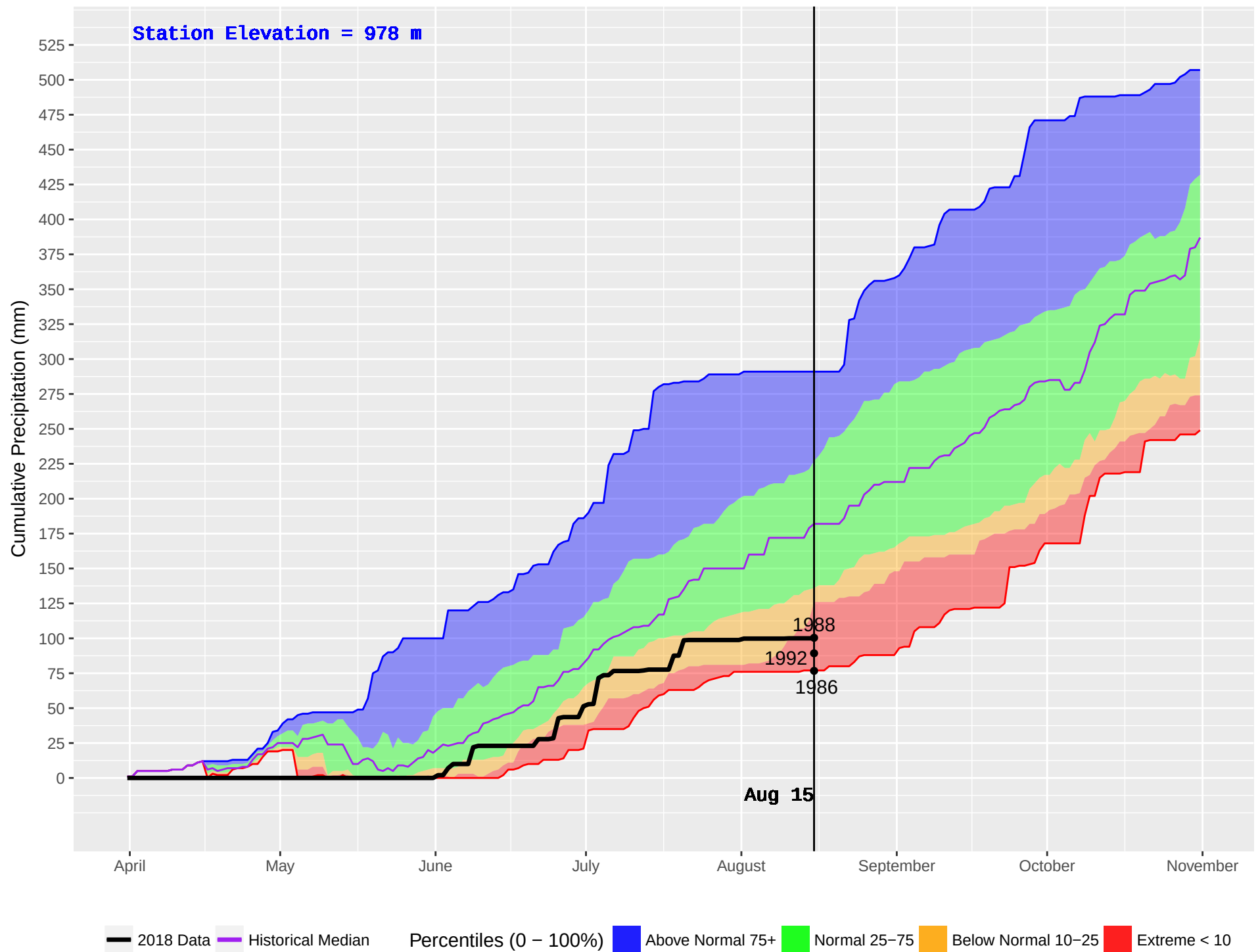
NILKITKWA (172) : Historical (1986–2016) and Current (2018) Daily Cumulative Precipitation
