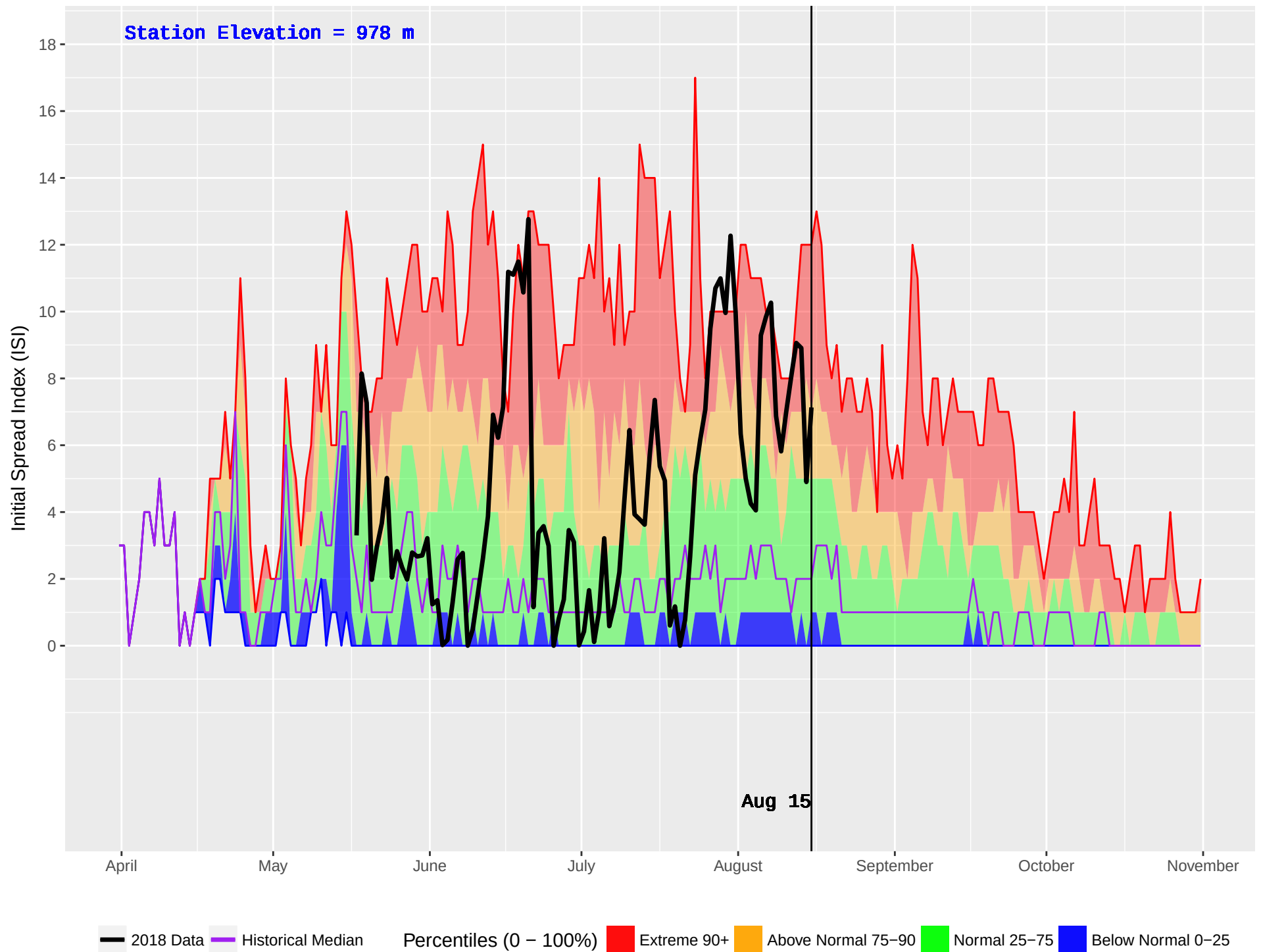
NILKITKWA (172) : Historical (1986–2016) and Current (2018) Daily Initial Spread Index (ISI)
